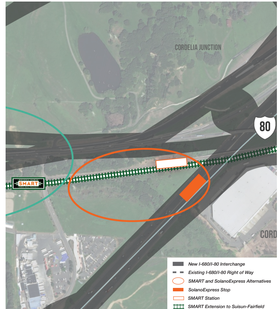
Figure 18: Red Top Road at I-80 Conceptual Design
