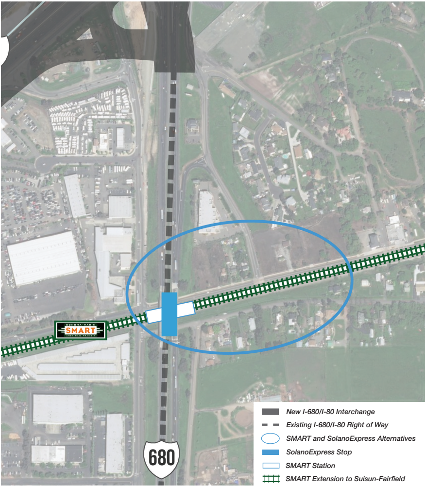
Figure 19: Cordelia Road/Lopes Road Conceptual Design
