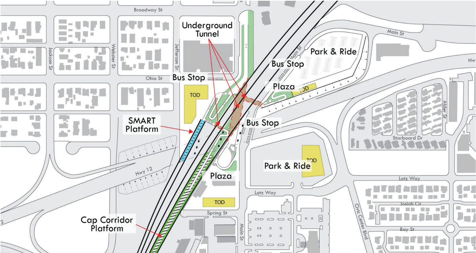
Figure 8: Plan view, Suisun-Fairfield Station Improvements
