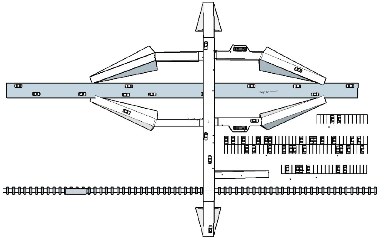
Figure 27: Option Five (Red Top Road at Highway 12) Aerial view
