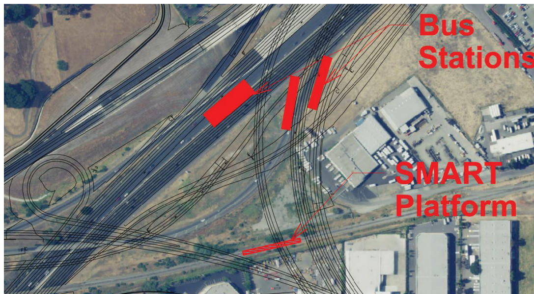
Figure 22: Option One SMART Platform and Express Bus Station Alignments
