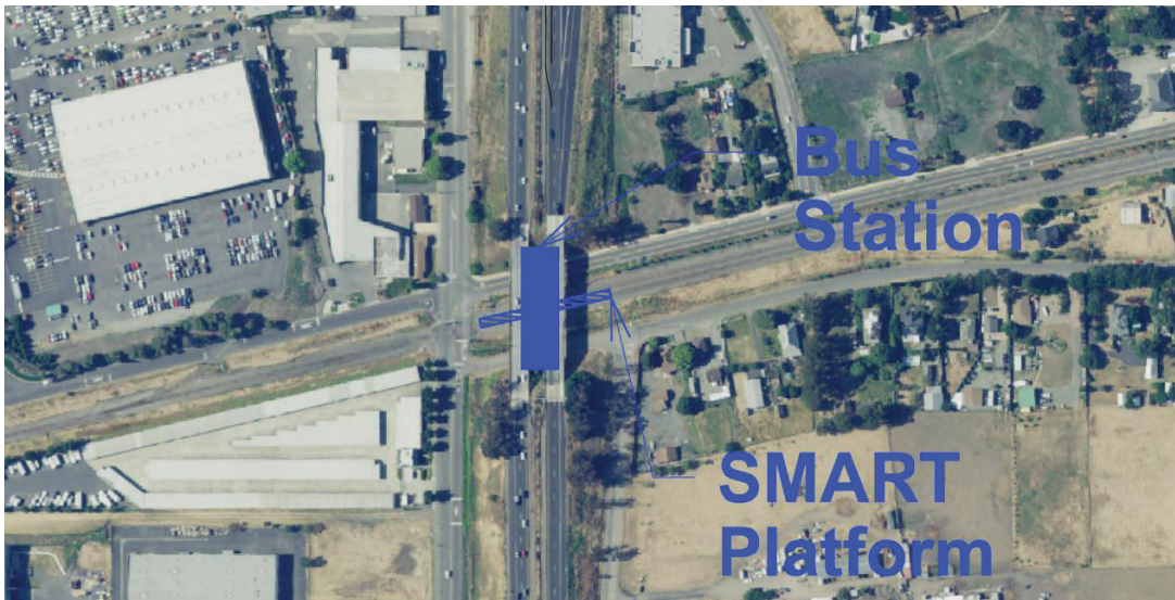
Figure 23: Option Two SMART Platform and Express Bus Station Alignments
