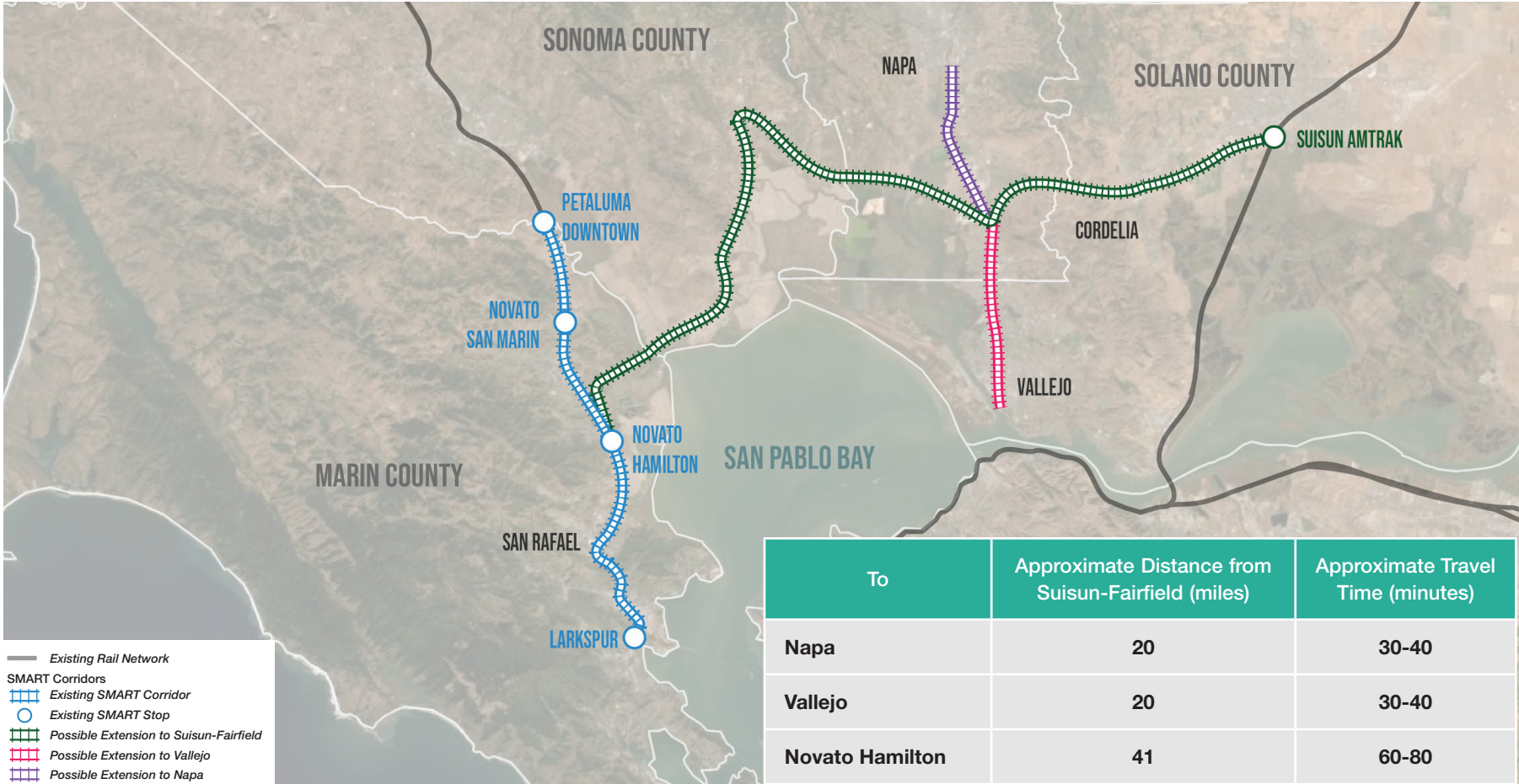
Figure 1: Proposed SMART Route from Novato to the Suisun-Fairfield Station
